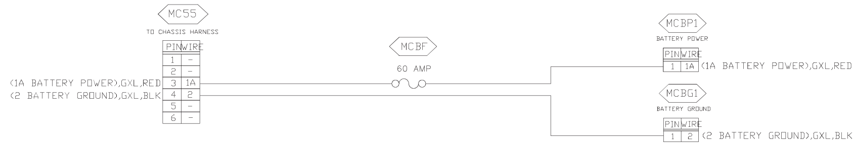
Schematic - 1479112 Battery Power Harness
